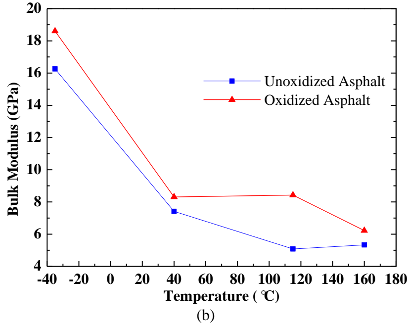
Figure 6.3 Isothermal compressibility (a) and bulk modulus (b) changes of unoxidized and oxidized asphalts under different temperatures
