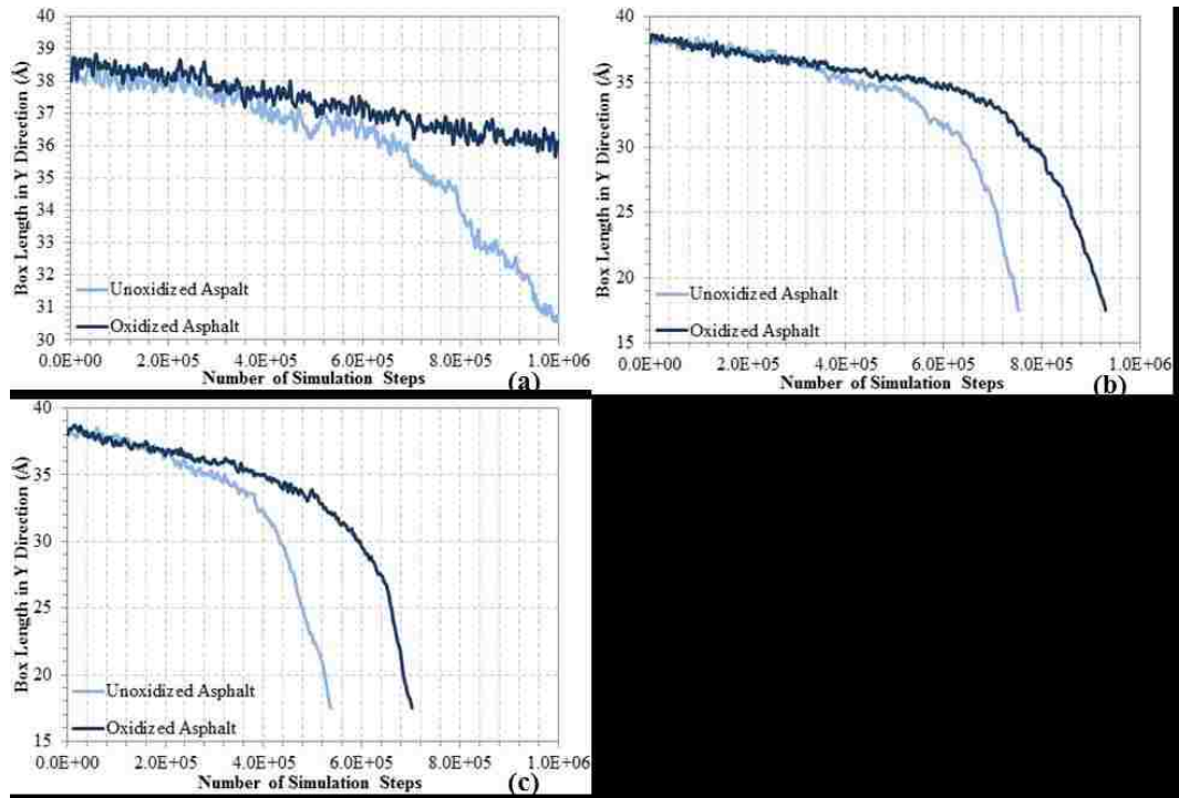
Figure 5.4 Comparison of unoxidized and oxidized asphalts under different compressive stress rates: (a) 284 \text{ GPa sec}^{-1} , (b) 709 \text{ GPa sec}^{-1} , and (c) 993 \text{ GPa sec}^{-1}
